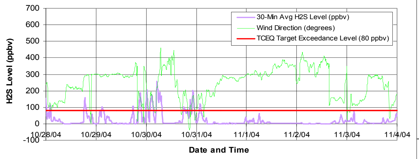
Figure B1l. H 2 S Levels (ppbv), CAMS 36, El Paso, 10/28/04-11/04/04
