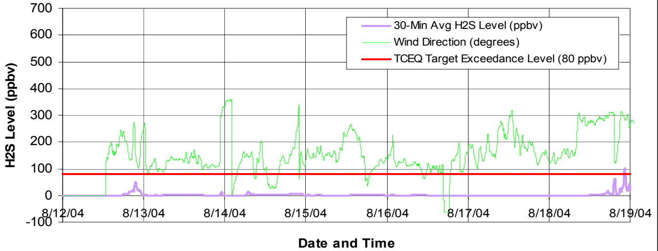
Figure B1a. H 2 S Levels (ppbv), CAMS 36, El Paso, 8/12/04-8/19/04
