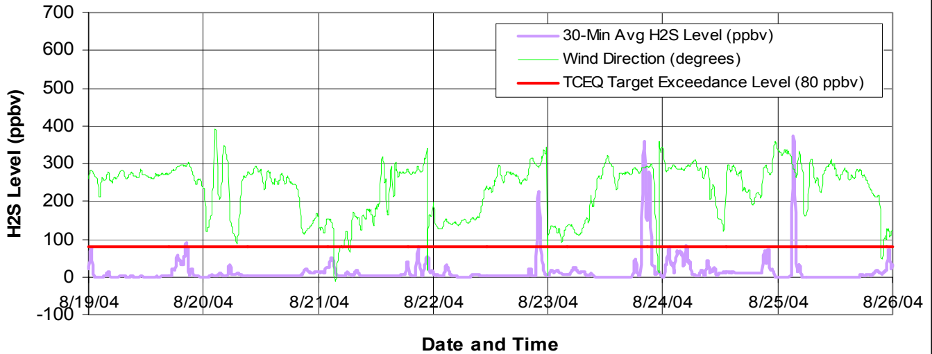
Figure B1b. H 2 S Levels (ppbv), CAMS 36, El Paso, 8/19/04-8/26/04
