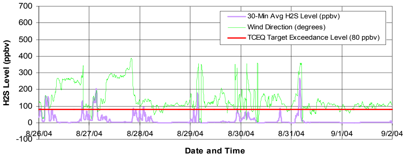
Figure B1c. H 2 S Levels (ppbv), CAMS 36, El Paso, 8/26/04-9/2/04
