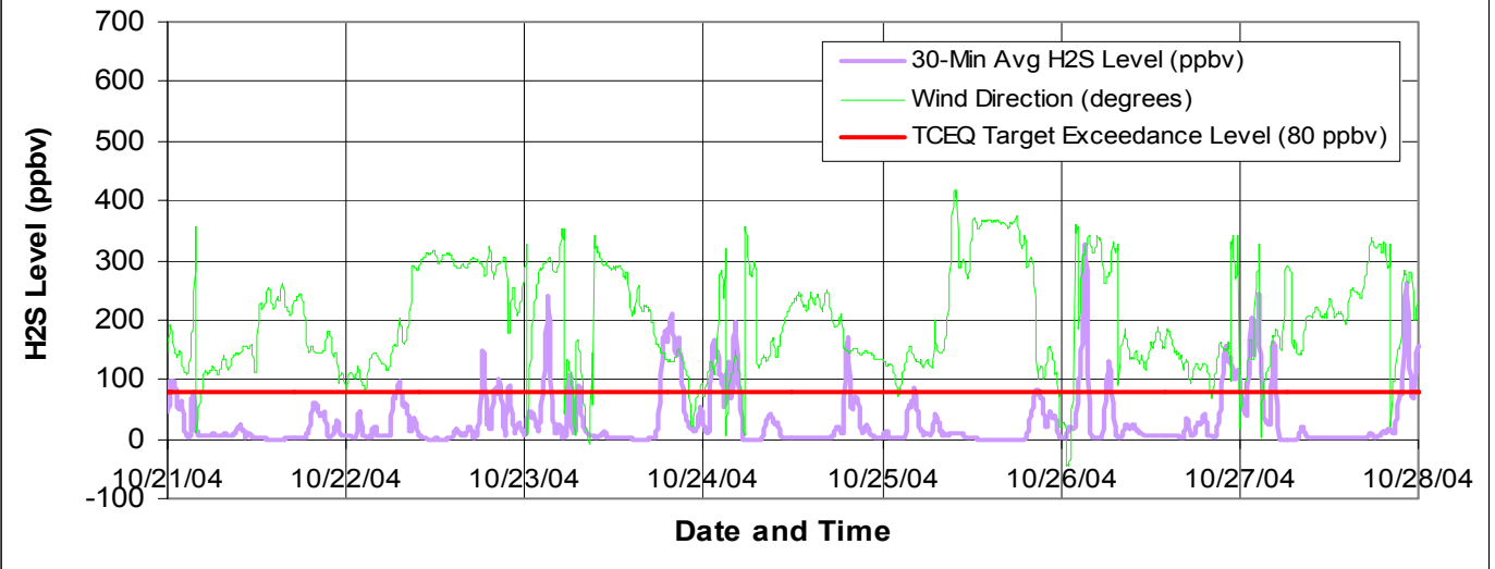
Figure B1k. H 2 S Levels (ppbv), CAMS 36, El Paso, 10/21/04-10/28/04
