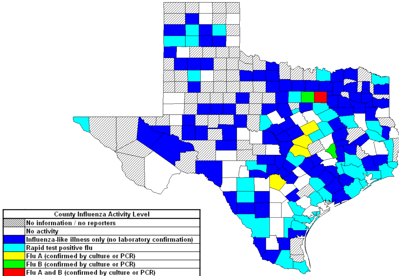
Figure 4: Texas Map Displaying the Highest Level of Influenza or ILI Activity Reported by County for the Week Ending Oct. 31, 2015 (MMWR Week 43)
