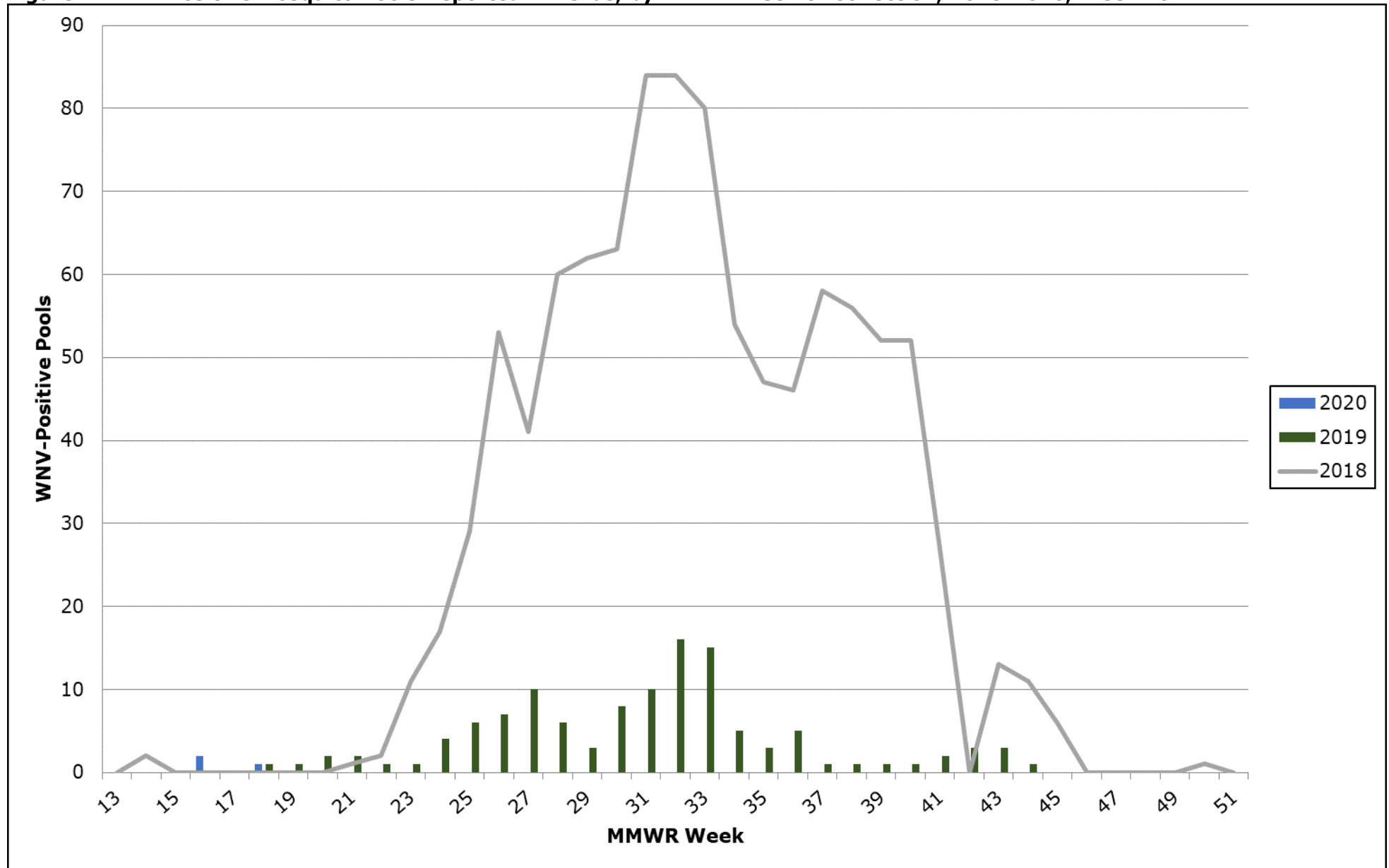
Figure 2. WNV-Positive Mosquito Pools Reported in Texas, by MMWR Week of Collection, 2018-2020, Week 20
