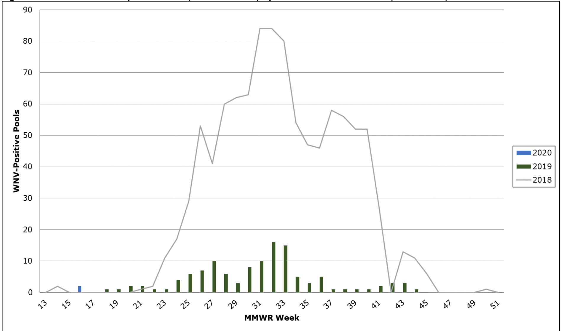
Figure 2. WNV-Positive Mosquito Pools Reported in Texas, by MMWR Week of Collection, 2018-2020, Week 18
