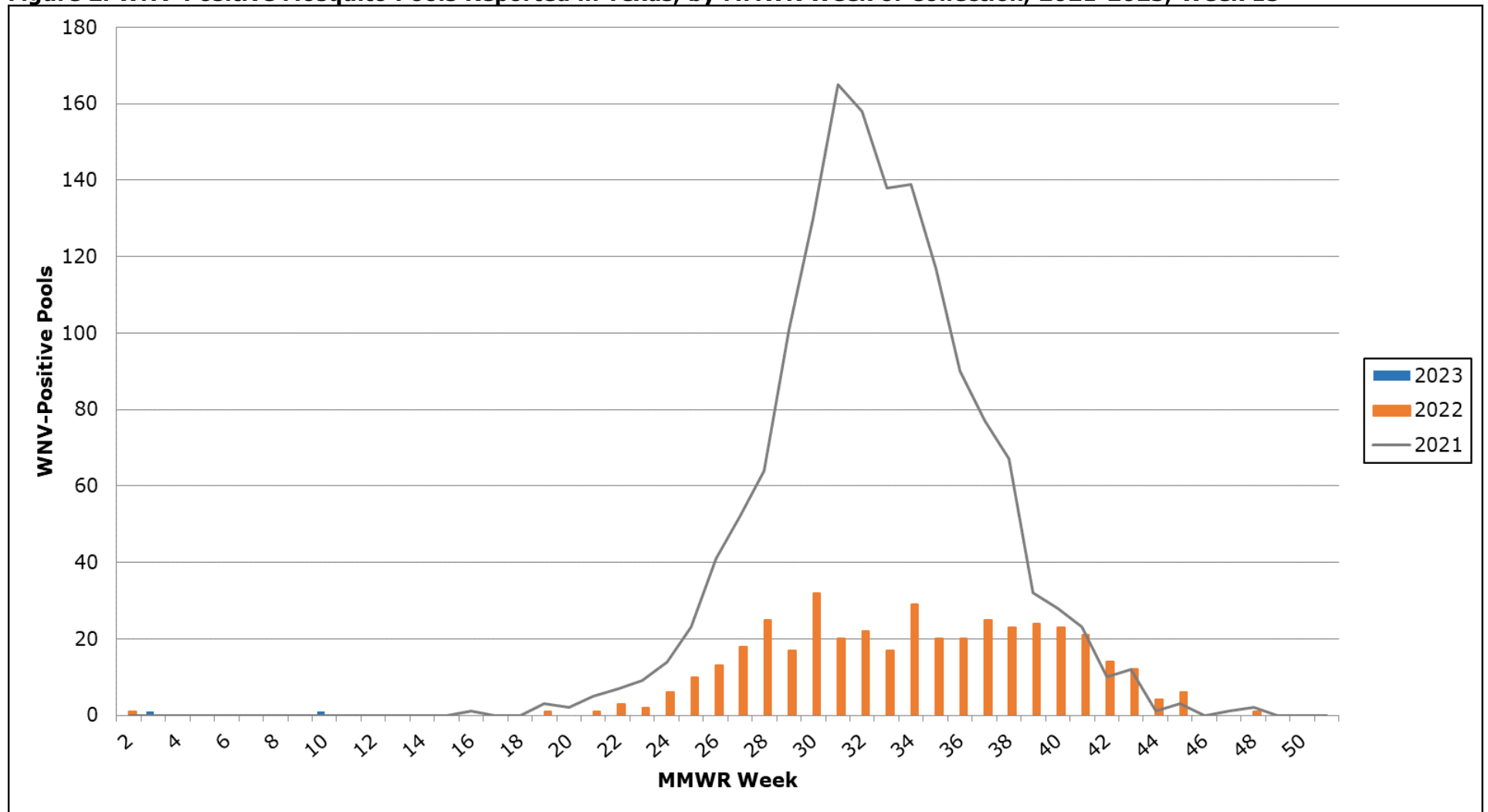
Figure 2. WNV-Positive Mosquito Pools Reported in Texas, by MMWR Week of Collection, 2021-2023, Week 15
