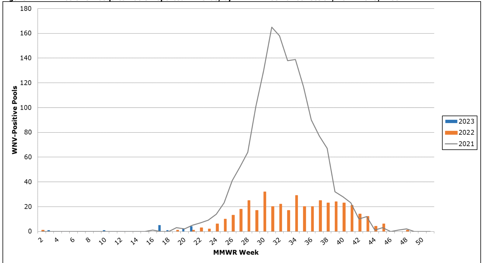
Figure 2. WNV-Positive Mosquito Pools Reported in Texas, by MMWR Week of Collection, 2021-2023, Week 22
